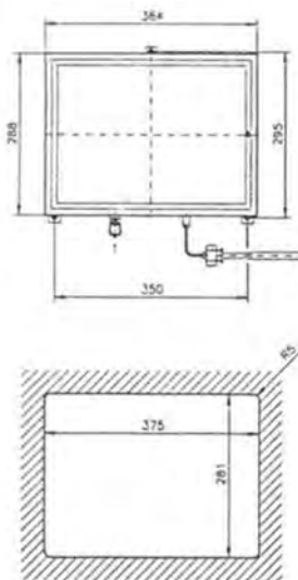
Double and triple recorder
